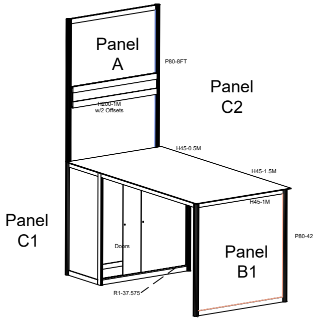
1 Isometric View :
