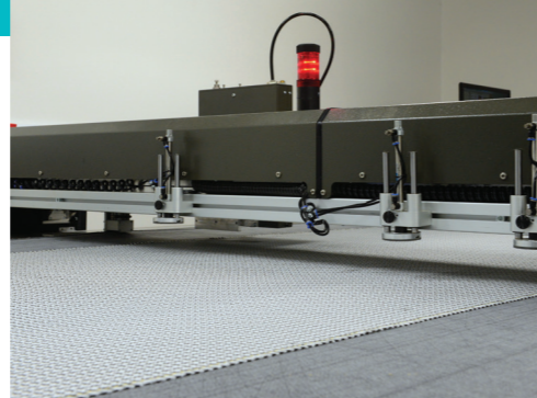
▲ Ply cutter for dry fabrics and preregs.
