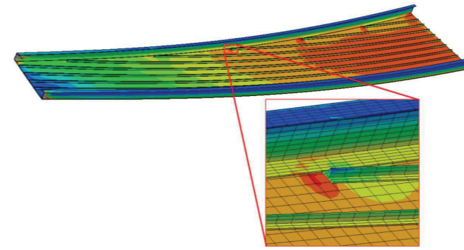
▲ We have the capability to embed local, detailed, models into larger, component scale models to predict the elastic and failure response.
