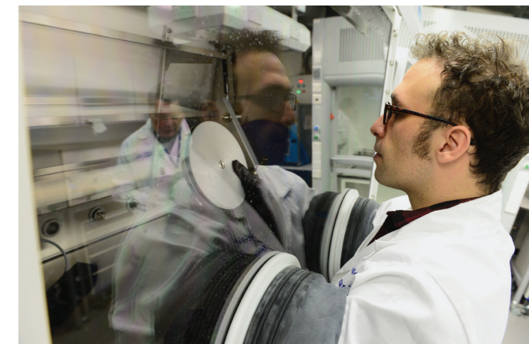
▲ We have glove box facilities to assemble multifunctional structural power materials in a moisture and oxygen free environment.
