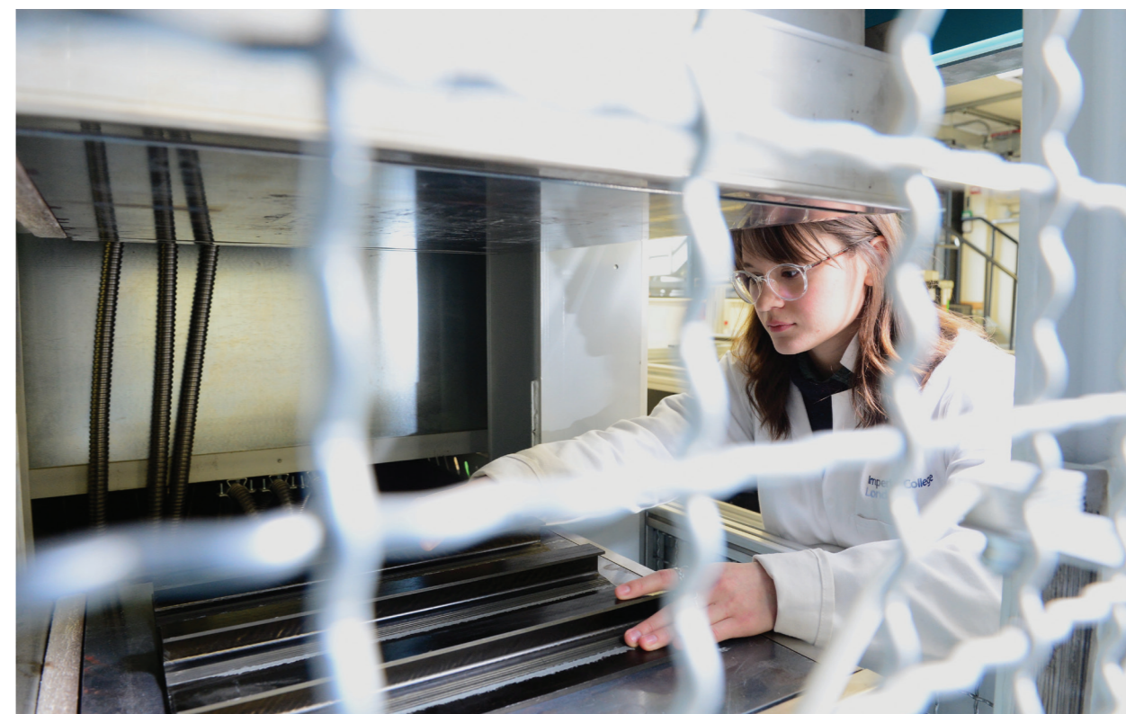
▼ With a maximum temperature of 4000° C, our custom made hydraulic press can not only be used to press mould and cure thermoset materials but also process high performance thermoplastics.
