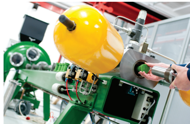
▲ Loading the gas gun to characterise high rate performance of composites.
