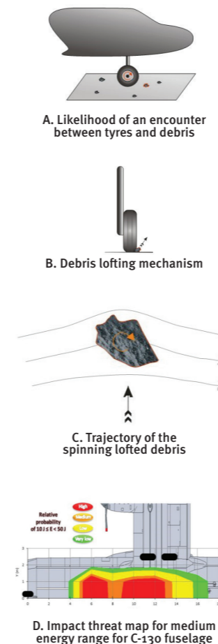
▲ Phases of the runway debris lofting process.
